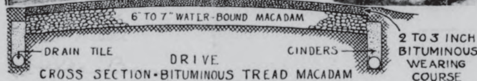
Roadbed as built by The Allied Products Co., compared with ordinary roadbed
